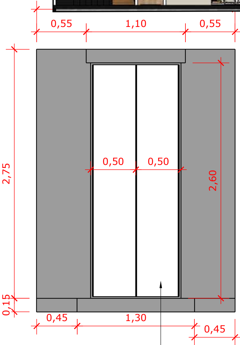
VISTA FRONTAL
