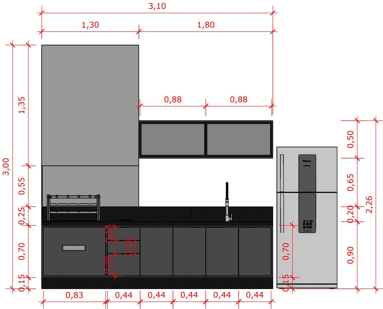
VISTA FRONTAL
