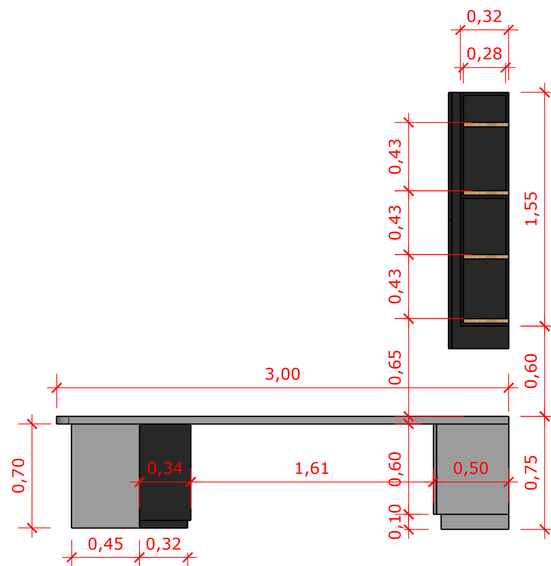
VISTA FRONTAL
