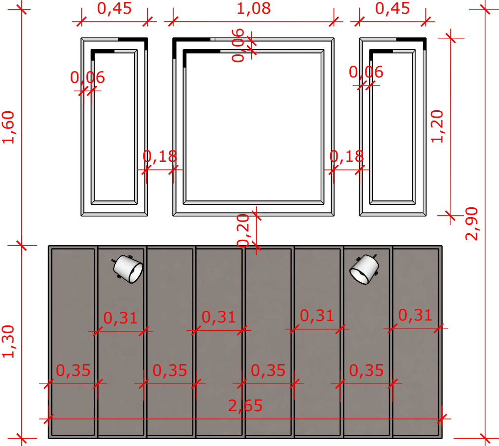
VISTA FRONTAL
