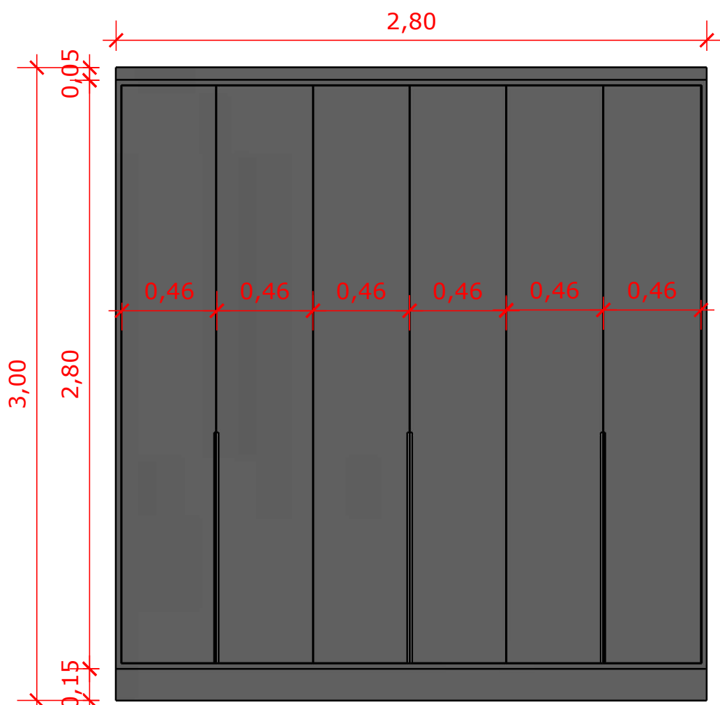
VISTA FRONTAL
