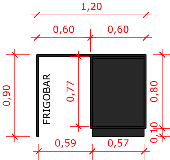
VISTA FRONTAL
