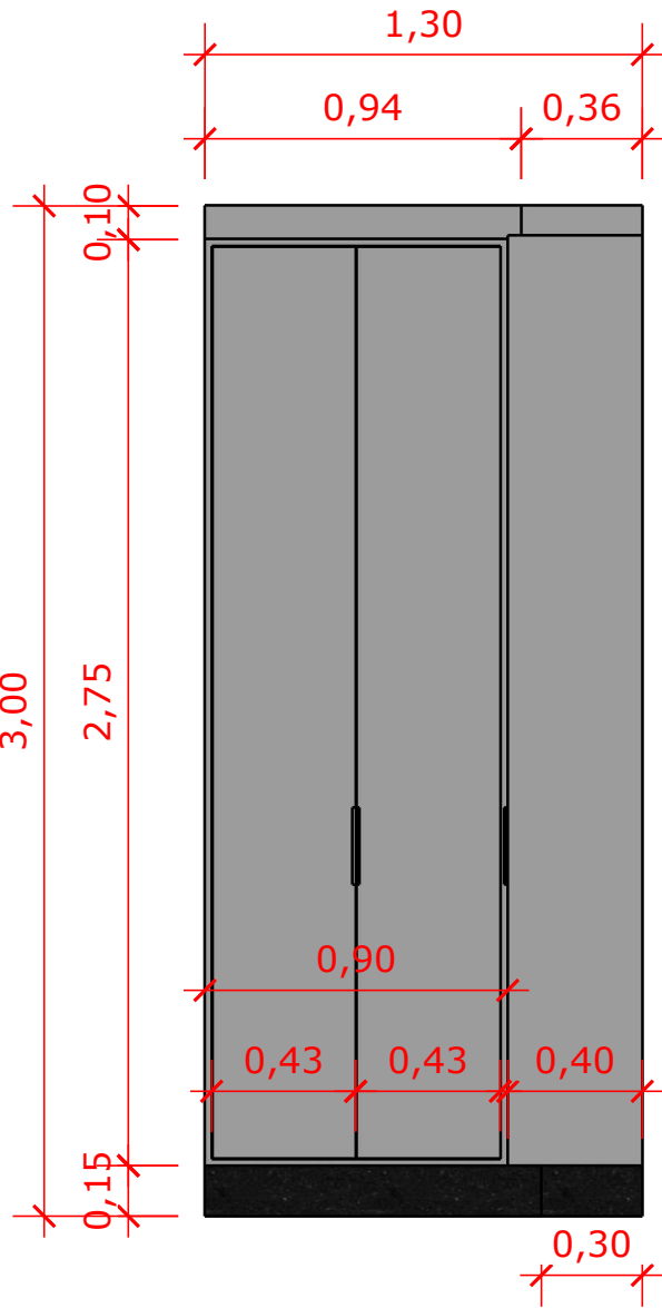
VISTA FRONTAL
