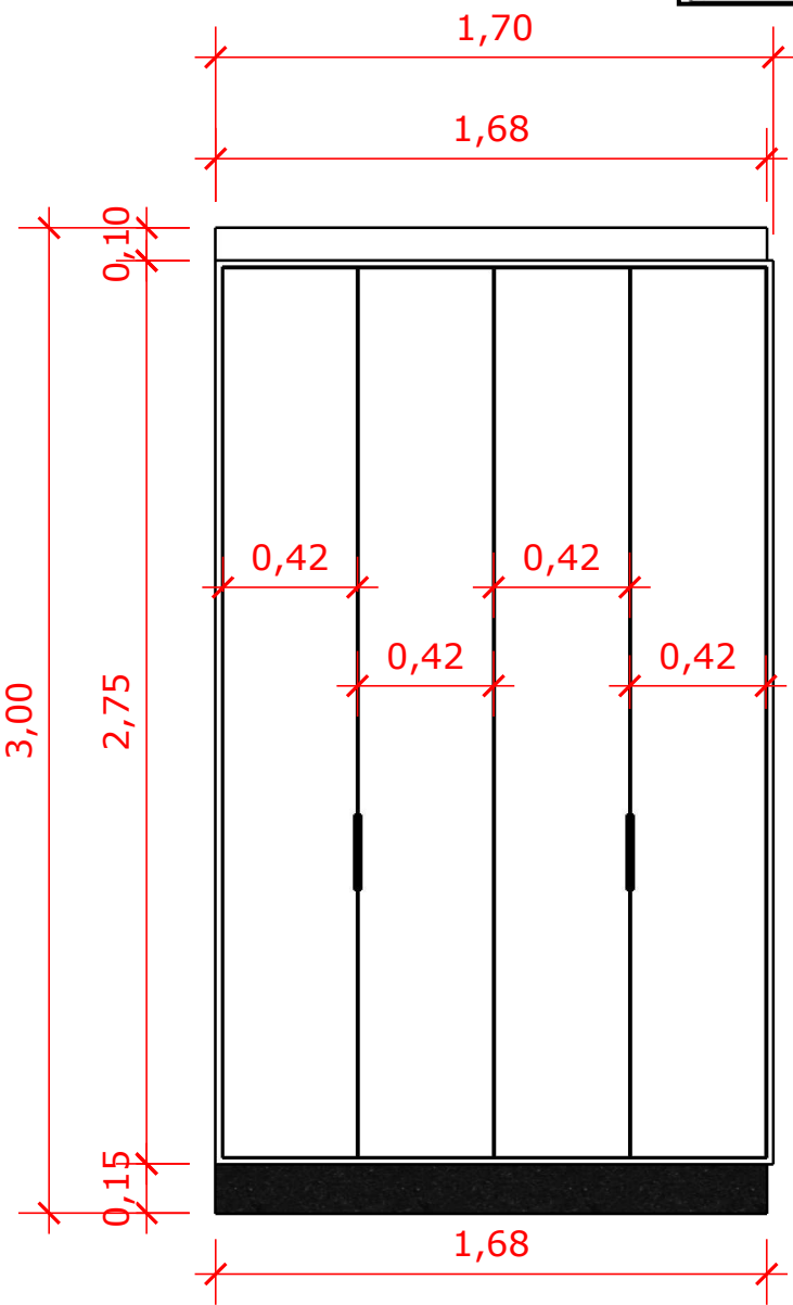
VISTA FRONTAL
