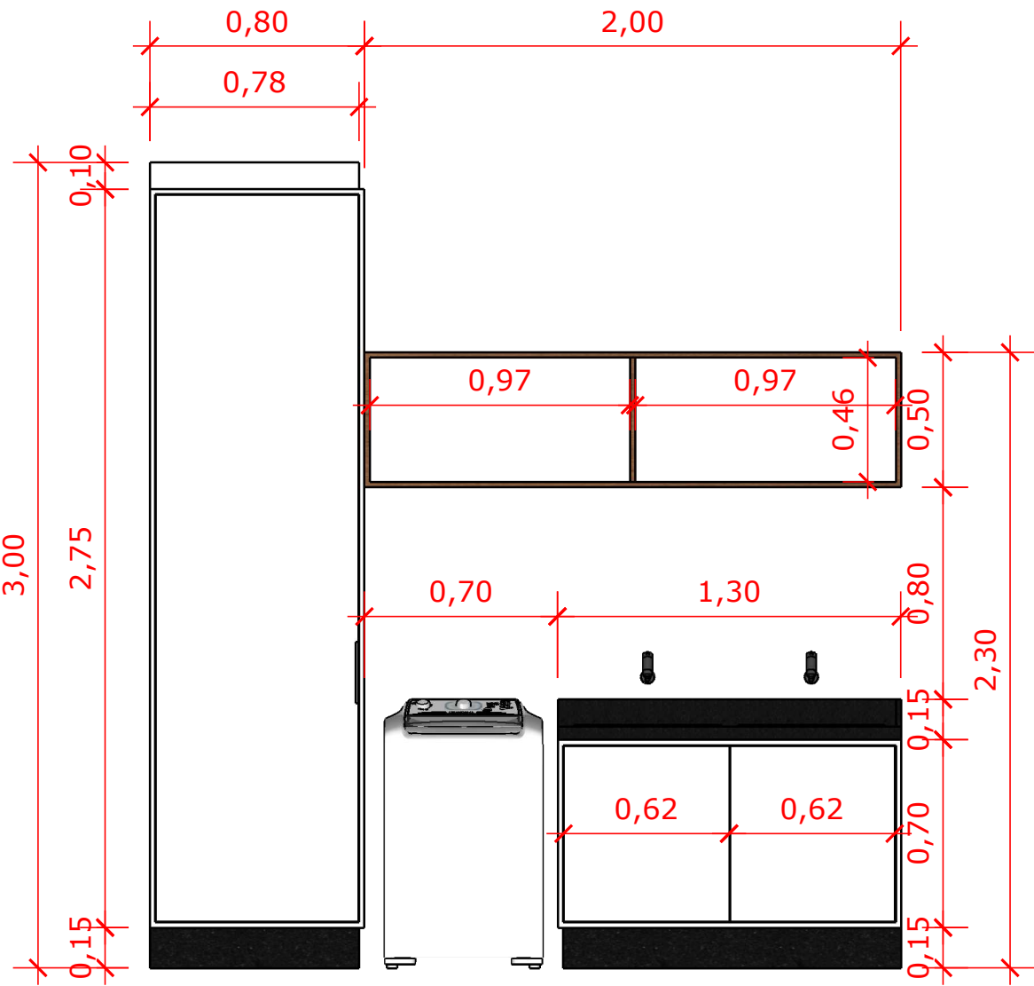
VISTA FRONTAL
