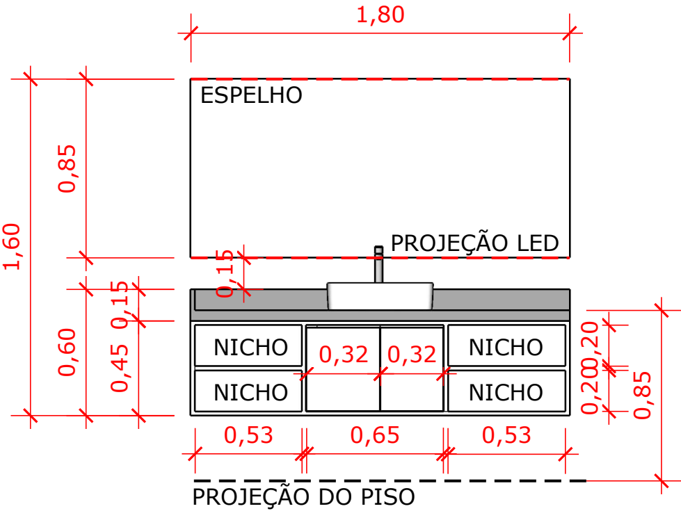
VISTA FRONTAL
