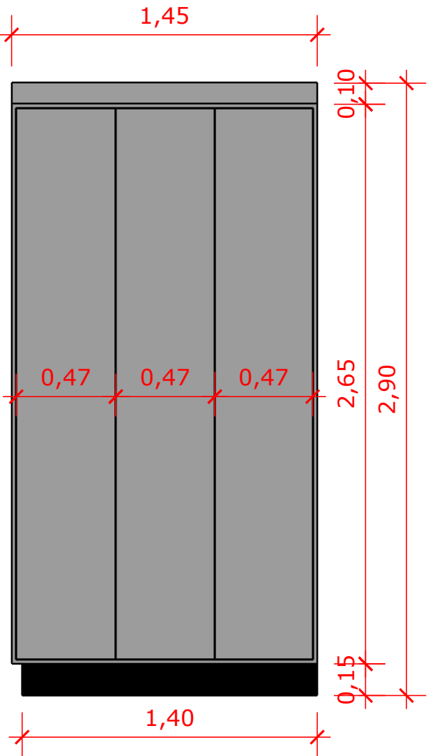
VISTA FRONTAL
