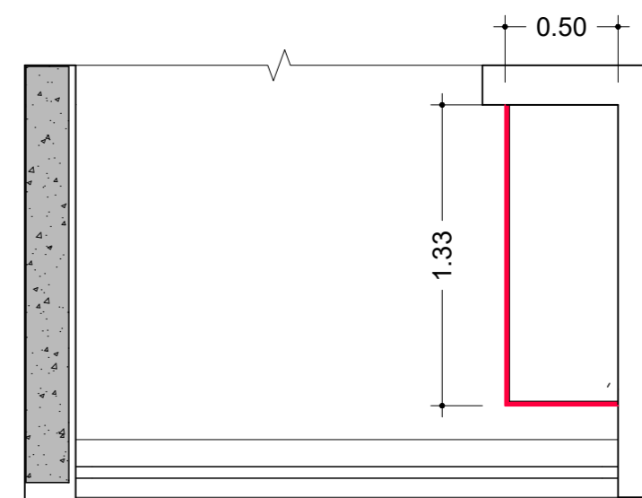
BASE - MARMORARIA VARANDA
